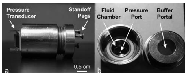
FIGURE 1 Direct membrane osmometer. (a) Side view of the stainless steel cylindrical device with microchip pressure transducer. (b) Polymeric solutions are injected into the fluid chamber, and the resulting pressure is measured at the pressure port. Ion and fluid exchange occurs through the buffer portal located in the lid of the device. Dialysis membrane and stainless steel wire-mesh backing for the membrane are not shown.
